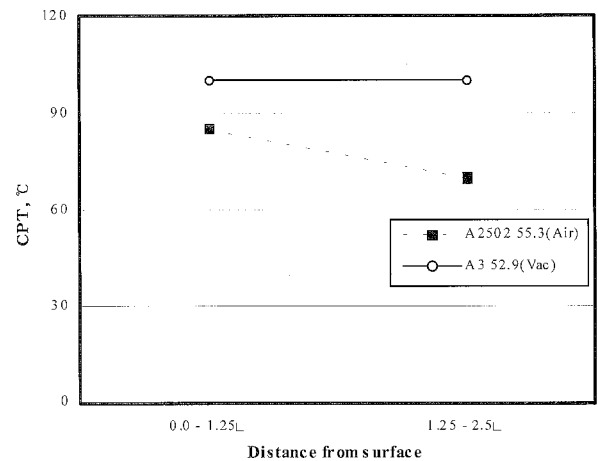
Fig. 1. Critical Pitting Temperatures of cast alloys in Green Death Solution.
