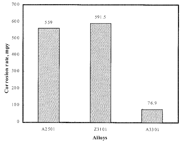
Fig. 18. Corrosion rates of alloys in 80 °C 80% H 2 SO 4 solution.
