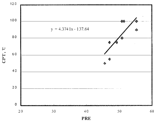
Fig. 6. CPT of air melted casts in 6% FeCl 3 solution
