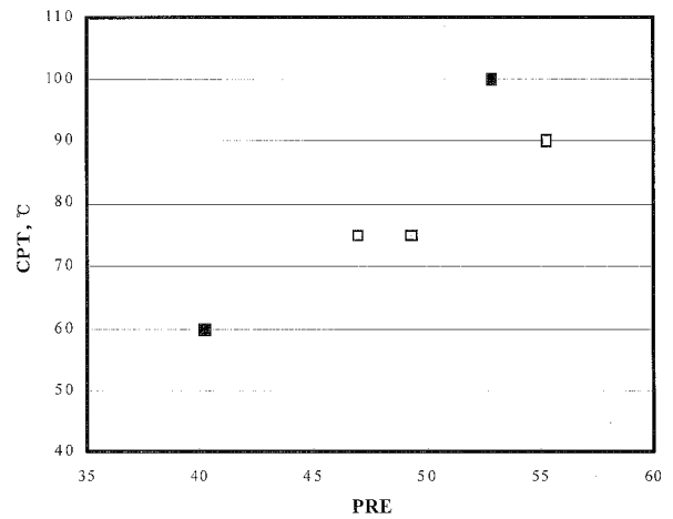
Fig. 8. CPT and PRE of representative air/vacuum melted cast alloys
