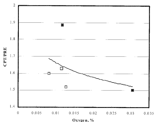
Fig. 10. CPT/PRE and oxygen concentration in alloys.
