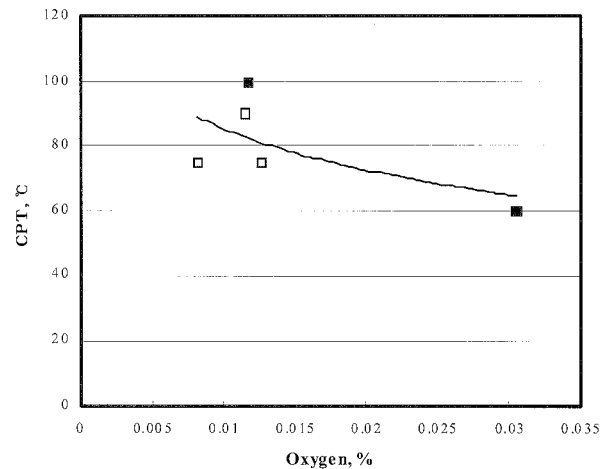
Fig. 9. The relation of CPT and oxygen concentration in alloys
