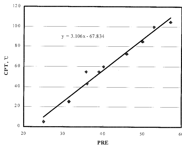
Fig. 4. CPT of vacuum melted casts in 6% FeCl 3 solution.
