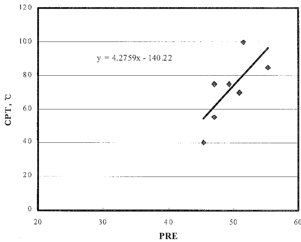
Fig. 7. CPT of air melted casts in Green Death Solution.
