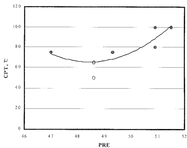
Fig. 12. Non-linear relation between PRE and CPT (6% FeCl 3 ) of alloys
