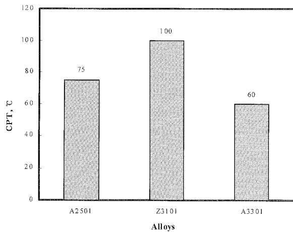
Fig. 15. CPTs of three alloys in Green Death Solution
