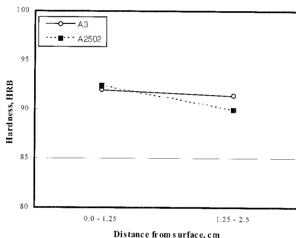
Fig. 3. Hardness variation according to the distance from the cast surface
