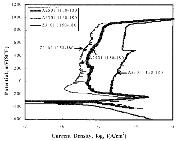
Fig. 16. APT curves of three alloys in 0.5 N HCl+1 N NaCl solution at 50 °C.
