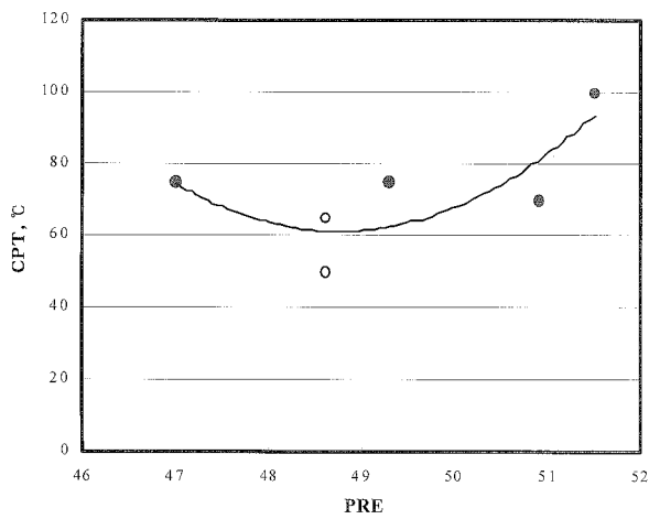
Fig. 14. Non-linear relation between PRE and CPT (Green Death Solution) of alloys
