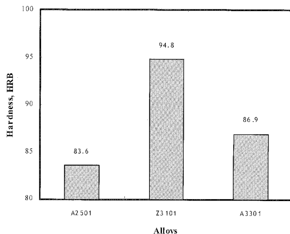
Fig. 11. Hardness variation according to Cr concentration in alloys
