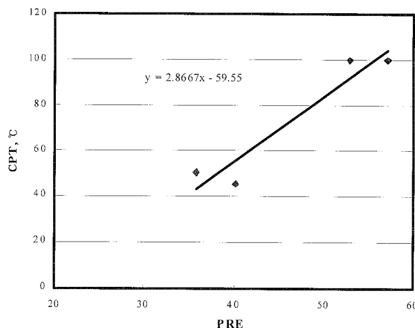
Fig. 5. CPT of vacuum melted casts in Green Death Solution
