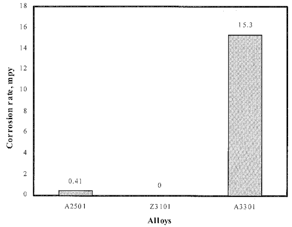
Fig. 17. Corrosion rates of alloys obtained from 1.5% HCl solution.
