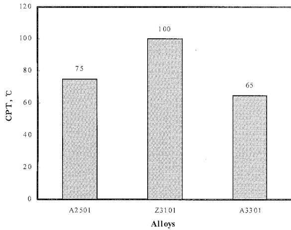
Fig. 13. CPT of alloys in 6% FeCl 3 solution
